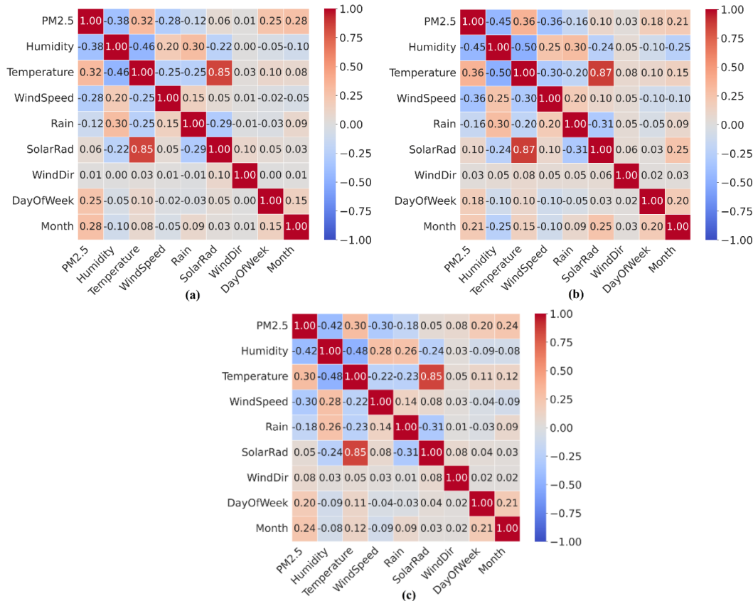
Figure 1. Spearman correlation matrix between pollutant and meteorological variables at stations: (a) Sajjad, (b) Torogh, and (c) Vila
