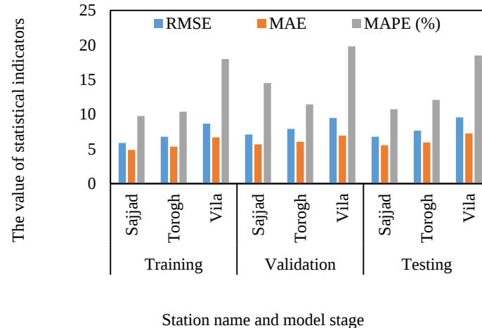
Figure 2. Comparison of MLP model performance indicators during the training, validation, and testing phases at the three monitoring stations
