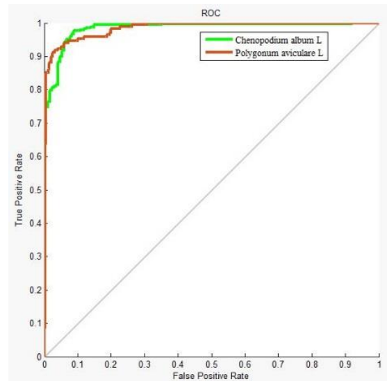
Figure 2. The ROC curve during the testing phase for the hybrid ANN-bee colony algorithm classifier
