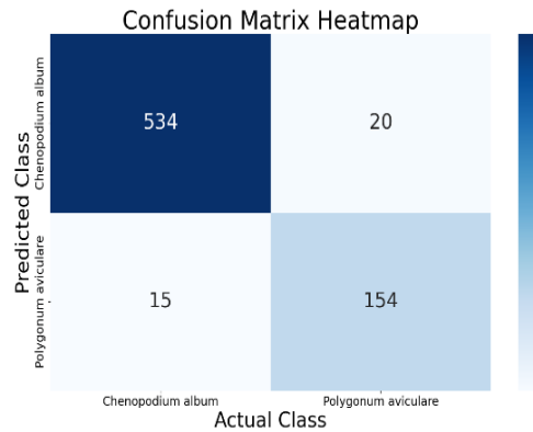
Figure 1. Test data classification using the hybrid neural network - bee algorithm classifier
