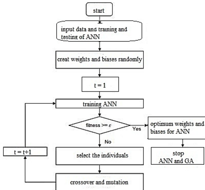
Figure 2. Block diagram of the combination of artificial neural networks and genetic algorithms
